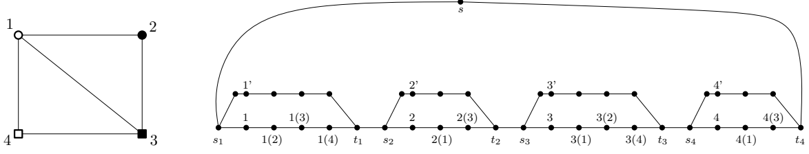
Figure 7: Example of the reduction in Theorem 8. Left: the original graph H . Right: the graph G_H . For problem (a) in Theorem 8, the reduction asks for a cycle through s that is in compliance with \mathcal{F}_{G_H} = \{\{1(2), 2(1)\}, \{2(3), 3(2)\}, \{3(4), 4(3)\}, \{4(1), 1(4)\}, \{1(3), 3(1)\}\} . For problem (b) in Theorem 8, the reduction asks for a cycle in compliance with \mathcal{F}_{G_H} \cup \{\{1, 1'\}, \{2, 2'\}, \{3, 3'\}, \{4, 4'\}\} .
