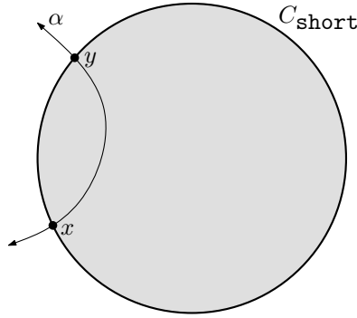
Figure 5: Figure for the proof of Lemma 5.
