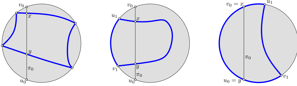
Figure 2: Left: an example for case (i) of Lemma 2. Center: an example for the first item in case (ii) of Lemma 2. Right: an example for the second item in case (ii) of Lemma 2.
