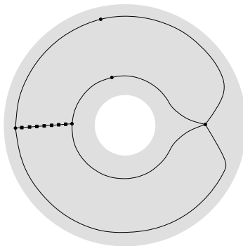
Figure 1: A graph embedded in an annulus. A shortest contractible cycle is strictly longer than a shortest contractible closed walk.
