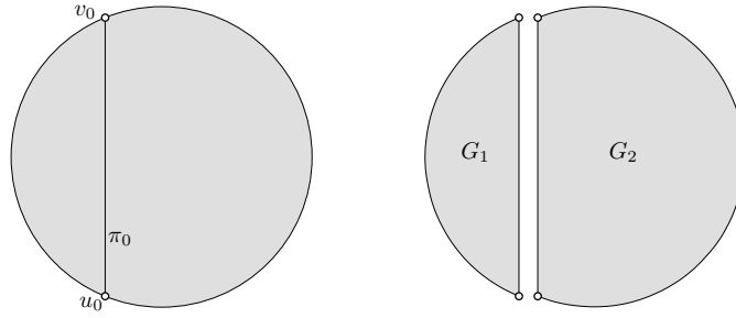
Figure 4: Left: the path \pi_0 . Right: the graphs G_1, G_2 obtained after cutting G along the arc \pi_0 .
