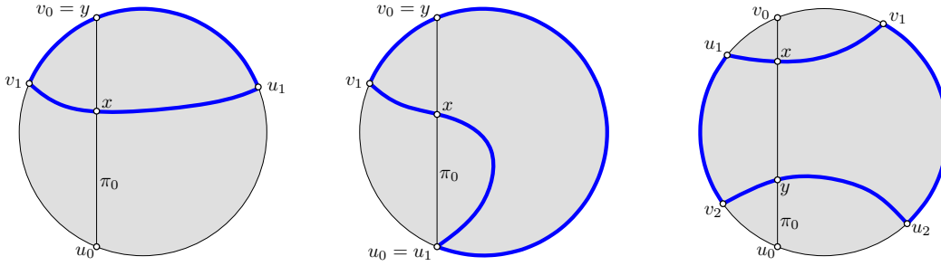
Figure 3: Left and center: examples for the third item in case (ii) of Lemma 2. Right: an example for case (iii) of Lemma 2.
