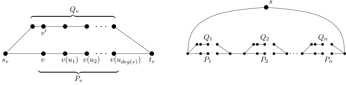
Figure 6: Reduction in Theorem 8.
