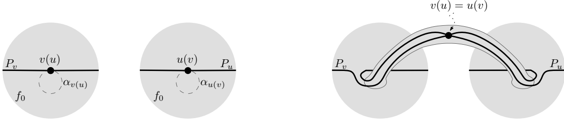
Figure 8: Illustration for the local transformation in the proof of Theorem 10. Left: part of the original graph G_H and two curves \alpha_{v(u)} and \alpha_{u(v)} . Right: part of the resulting surface \Sigma after adding the handle corresponding to the edge uv of H .
