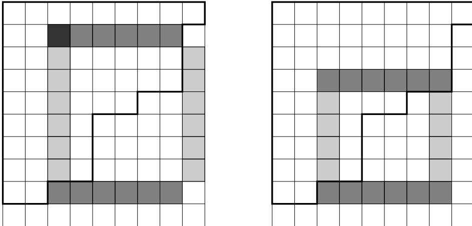
FIGURE 9. Hooks for the partition and its complement when \lambda = 988864442 .
