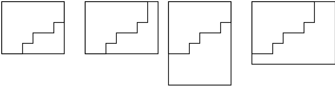
FIGURE 8. Complementary partitions of \lambda = 66532 with respect to (5, 6) , (5, 7) , (8, 6) and (6, 8) are 431, 54211, 666431, 865322, respectively.
