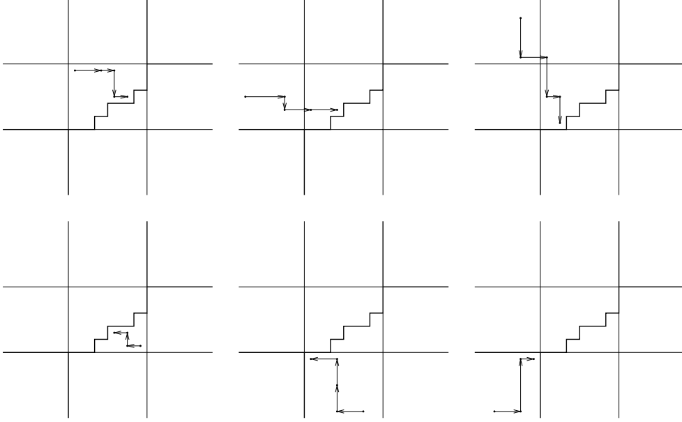
FIGURE 7. Examples of (weighted) hook walks for \lambda = 66532 .
