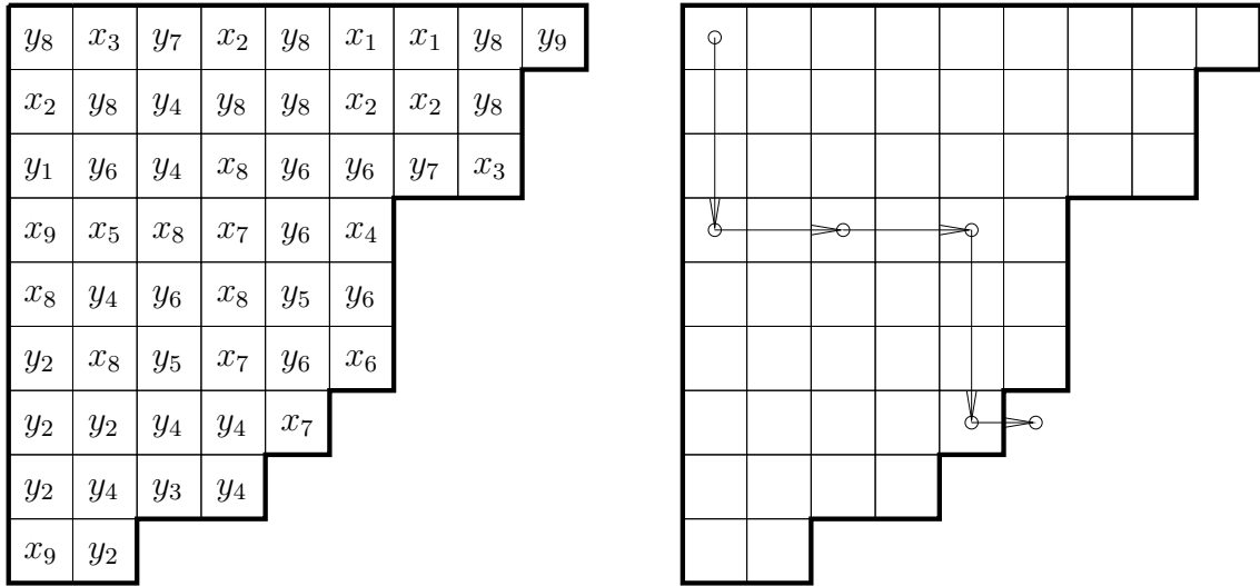
FIGURE 3. An example of an arrangement corresponding to the left-hand side of CWBR for \lambda = 988666542 ; the corresponding hook walk.
