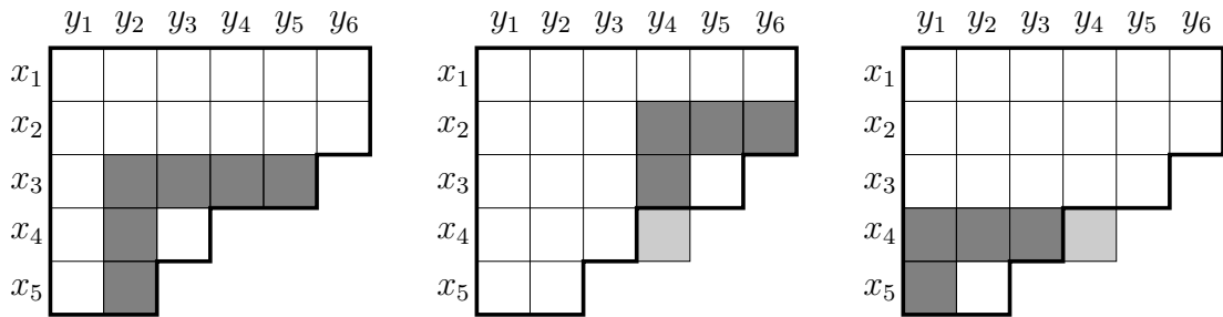
FIGURE 2. The term on the left-hand side of CWBR corresponding to the square (3, 2) is x_3 + x_4 + x_5 + y_2 + y_3 + y_4 + y_5 (left); the terms on the right-hand side of CWBR corresponding to the outer corner (4, 4) and the squares (2, 4) and (4, 1) are x_3 + y_4 + y_5 + y_6 (middle) and x_4 + x_5 + y_2 + y_3 (right).
