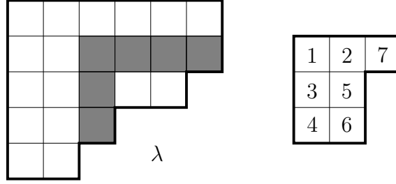
FIGURE 1. Young diagram [\lambda] , \lambda = 66532 , and a hook H_{23} with hook length h_{23} = 6 ; a standard Young tableau of shape 322.
