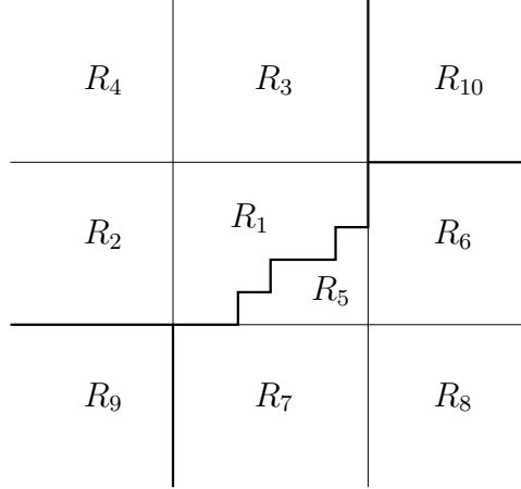
FIGURE 6. Division of the plane into regions R_1, \dots, R_{10} for \lambda = 66532 , with some lines in bold.
