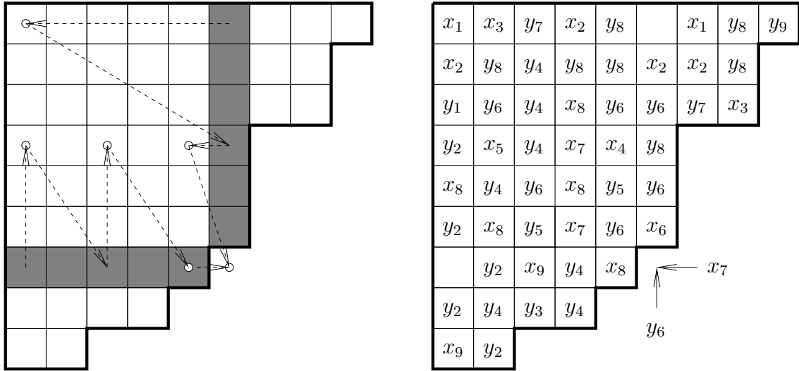
FIGURE 4. An example of the shift of labels for \lambda = 988666542 .
