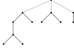
Fig. 4: The plane tree corresponding to a subpolytope.
